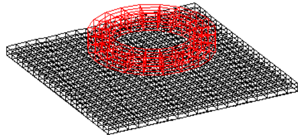
Figure 4. Maillage des parties actives
